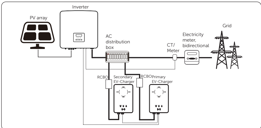
Figure 14-4 Parallel function - communication with inverter
