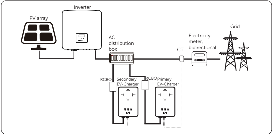
Figure 14-5 Parallel function - communication with CT
